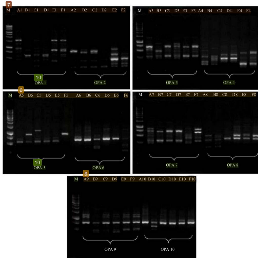
Fig. 4: Visualization of RAPD band pattern of 6 individuals O.c. toeantei with OPA primer 1-10
